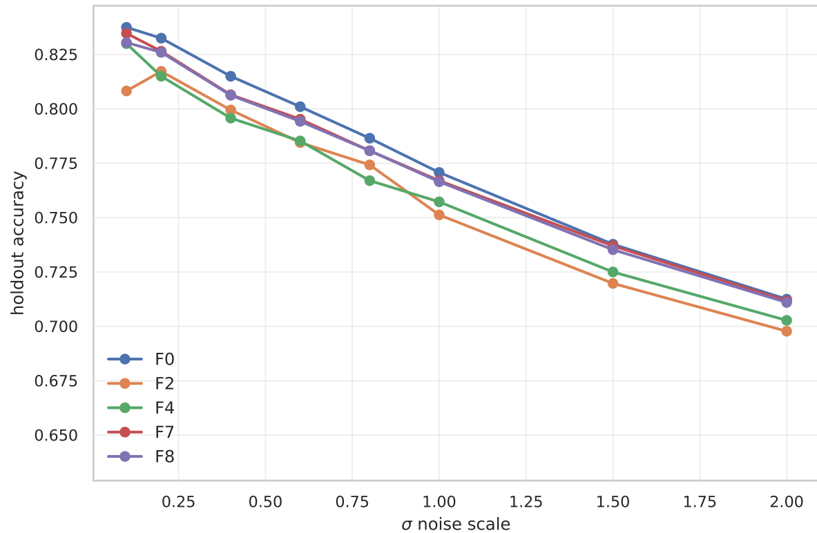
N1: holdout acc vs \sigma (Adam)
