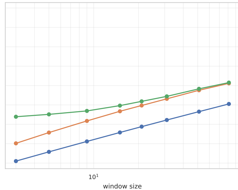
N4 Mixed
