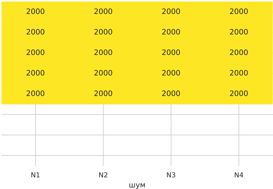
Adam
