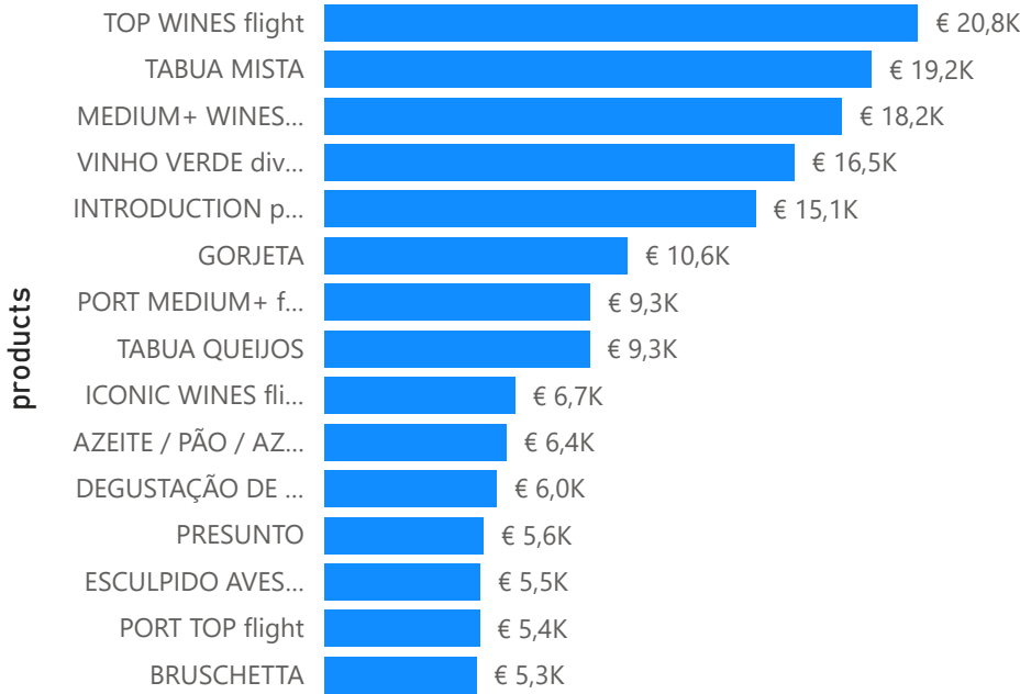
Gross revenue by products
