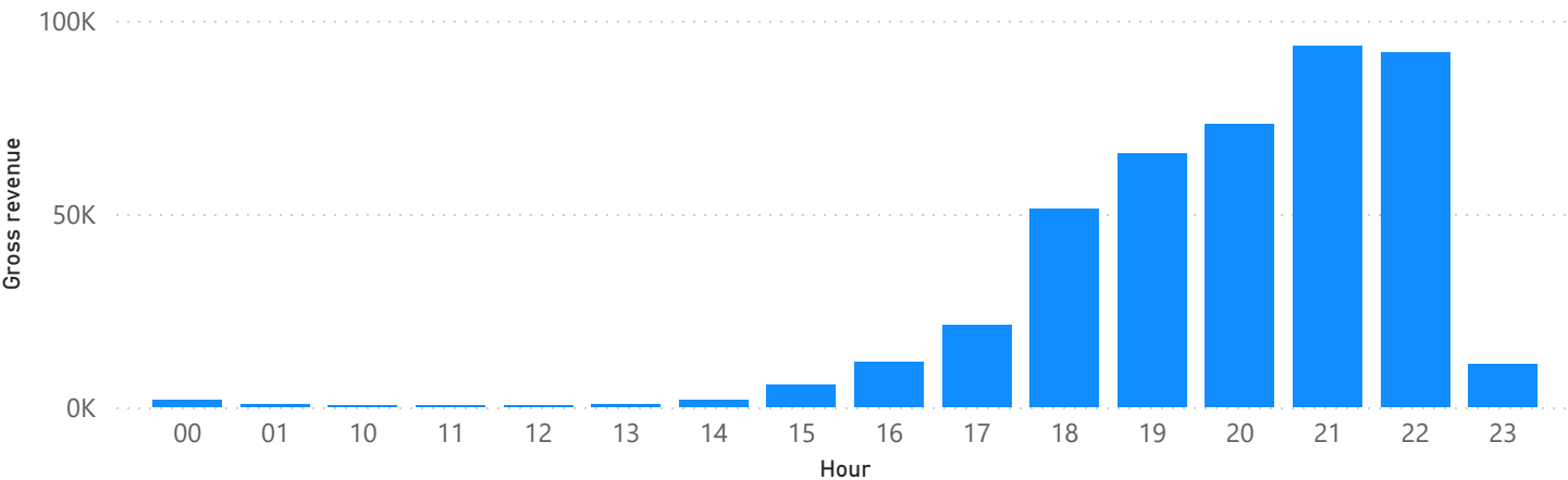
Gross revenue by Hour
