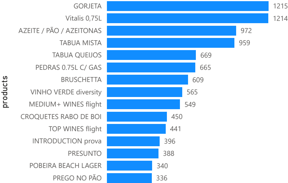
Total quantity by products
