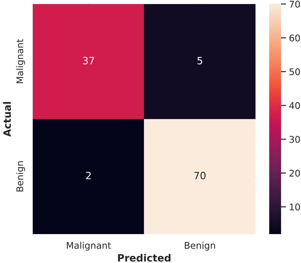
Decision Tree Confusion Matrix
