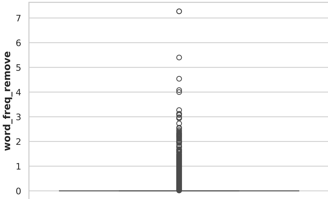
Boxplot of word_freq_remove
