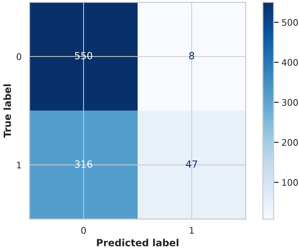
Confusion Matrix - Bernoulli NB
