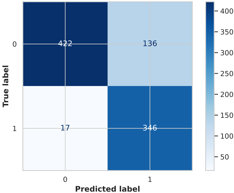
Confusion Matrix - Gaussian NB
