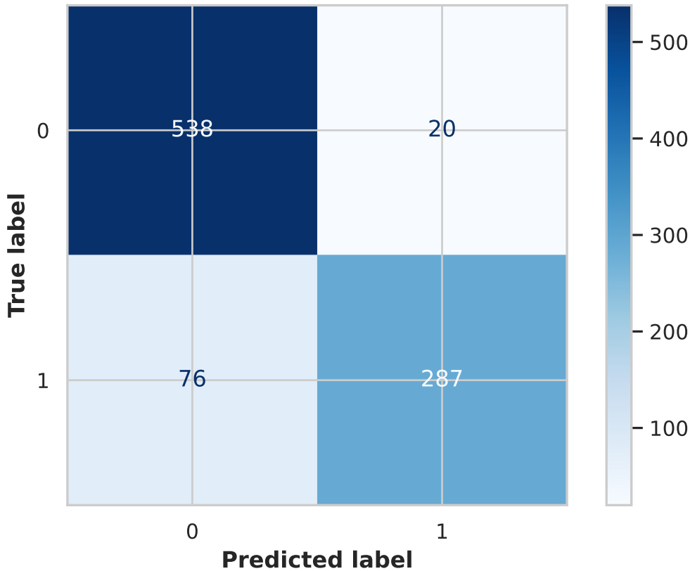
Confusion Matrix - Multinomial NB
