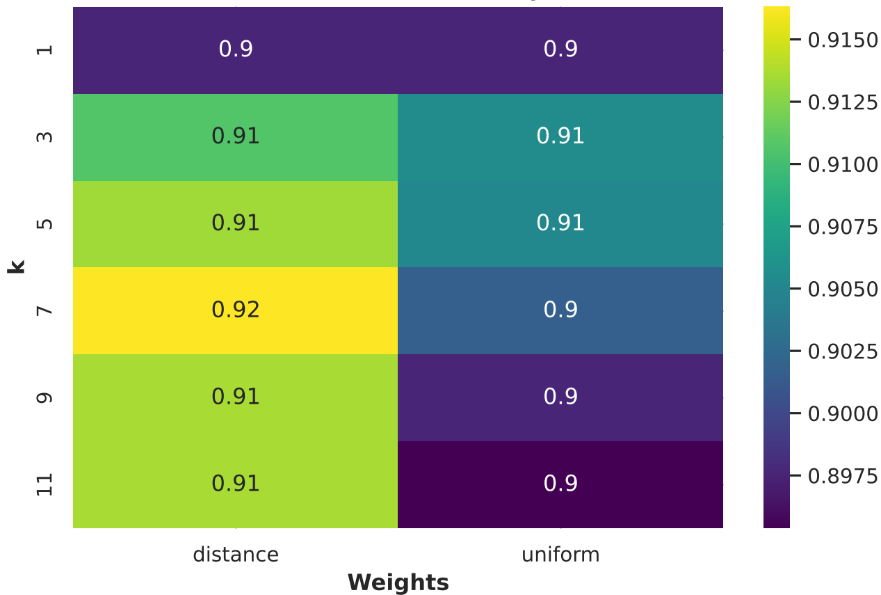
GridSearchCV Heatmap
