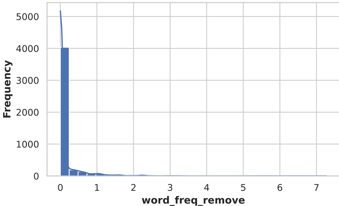
Histogram of word_freq_remove
