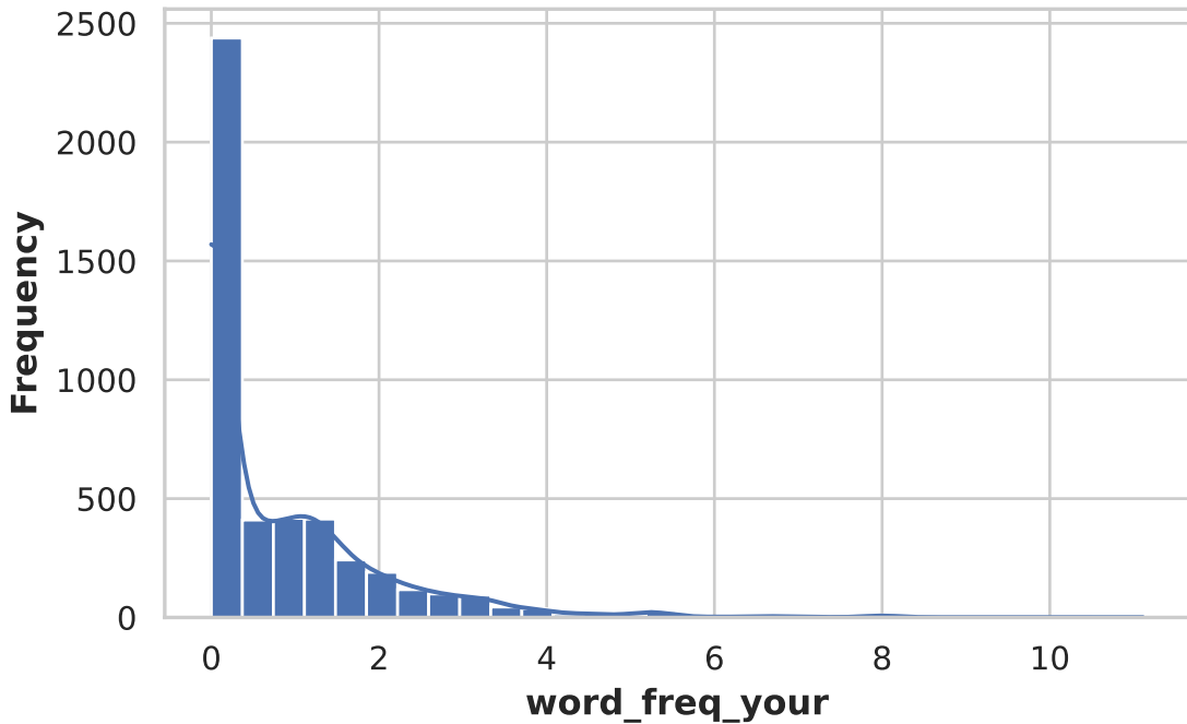
Histogram of word_freq_your
