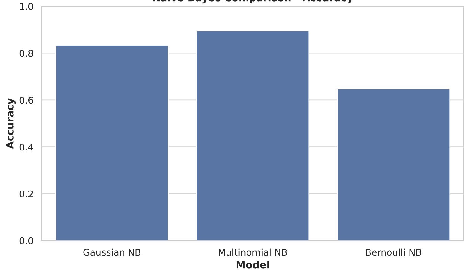
Naïve Bayes Comparison - Accuracy
