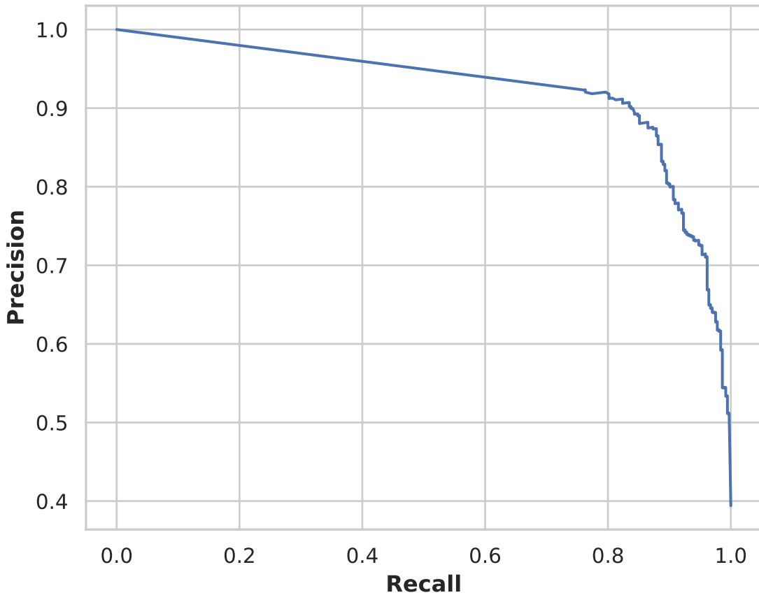
Precision-Recall Curve - Gaussian NB
