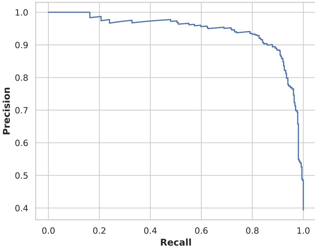
Precision-Recall Curve - Multinomial NB
