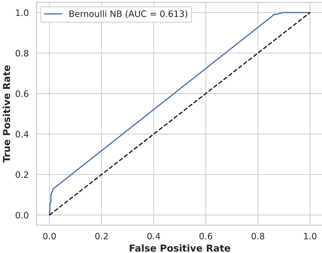
ROC Curve - Bernoulli NB
