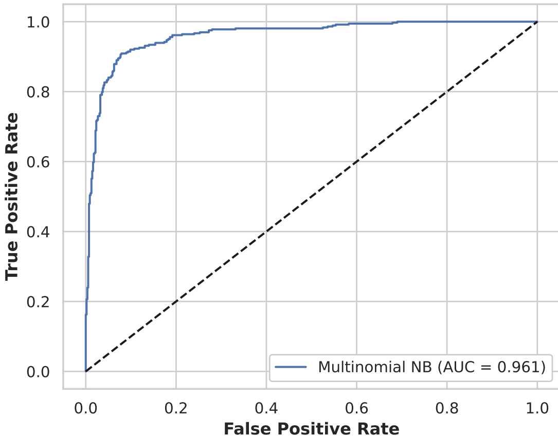
ROC Curve - Multinomial NB
