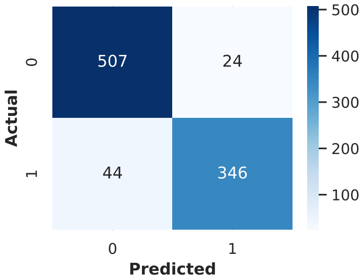
Linear Kernel Confusion Matrix
