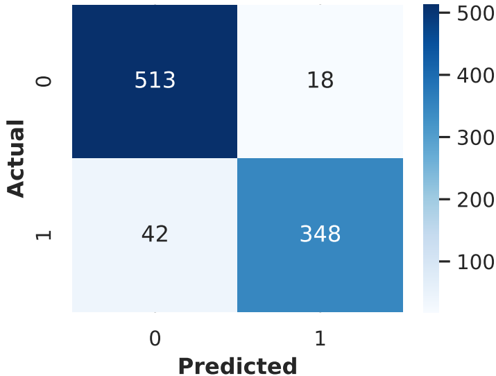
Rbf Kernel Confusion Matrix
