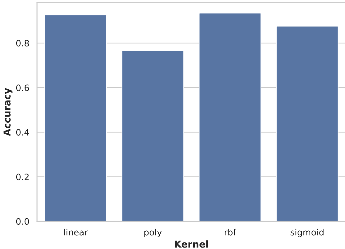
SVM Kernel Accuracy
