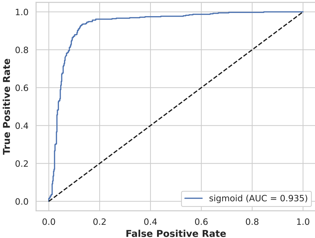
ROC Curves for SVM Kernels
