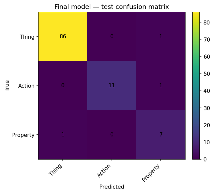
Figure 19 – Confusion matrix of the final model.
