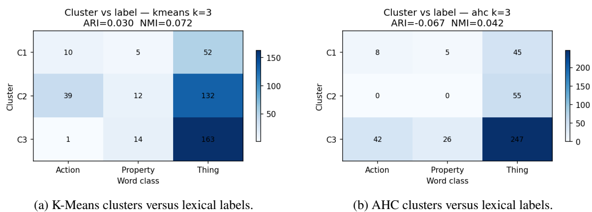
Figure 35 – Association between unsupervised clusters and the original lexical-semantic classes.
