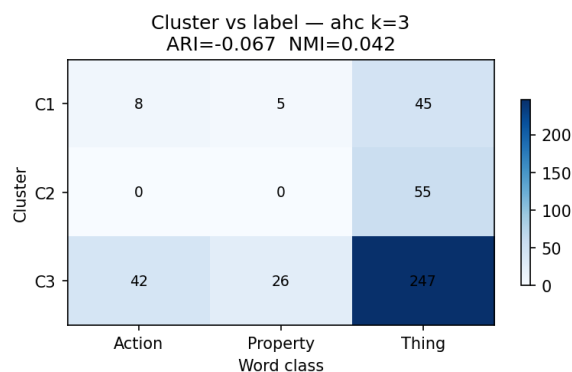
Figure 12 – Cluster-label correspondence heatmap, AHC K = 3 .
