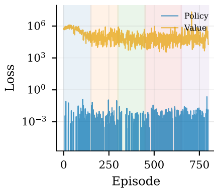
(e) Training Loss
