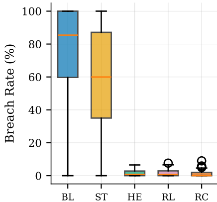
(b) BR Distribution
