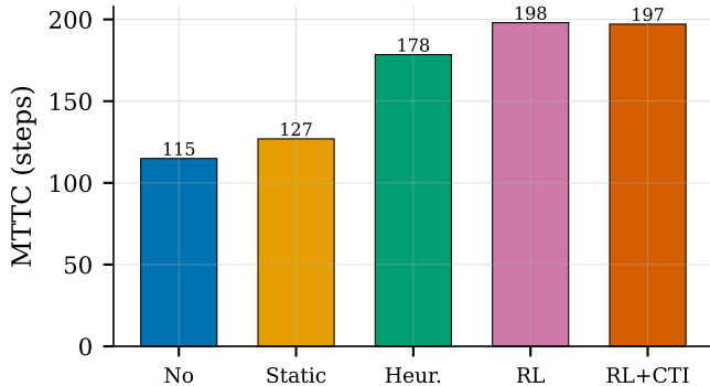
(a) Mean Time to Compromise
