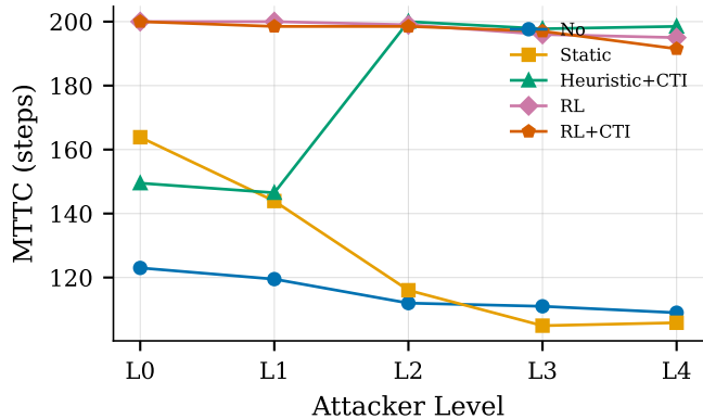
(b) MTTC by Attacker Level
