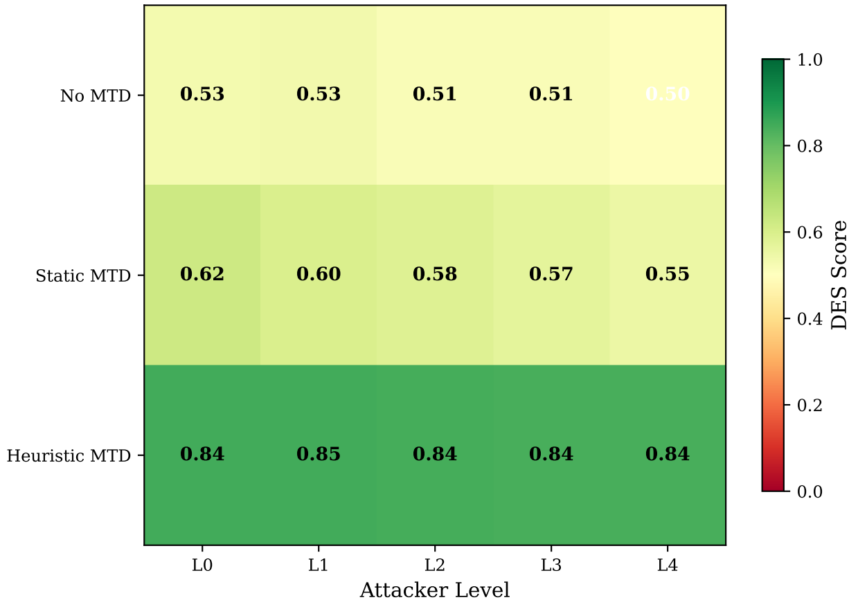
Defense Effectiveness Score (DES) Heatmap
