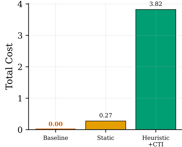
(f) Cost
