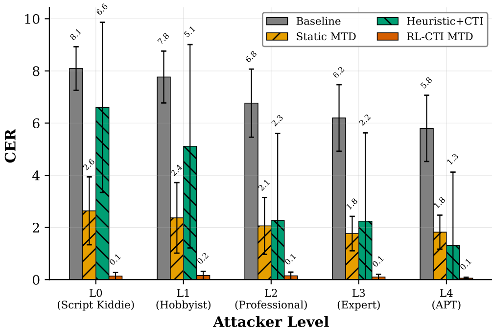
CER by Attacker Level
