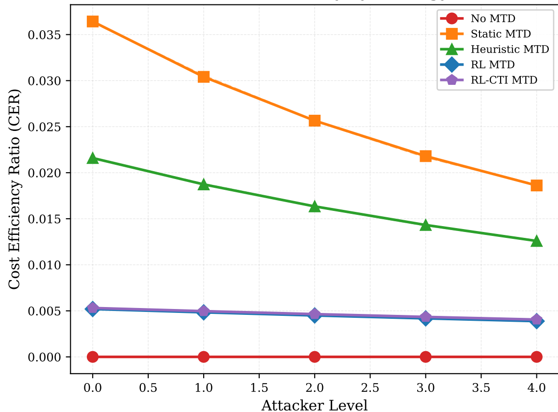
(b) Cost Efficiency by Strategy
