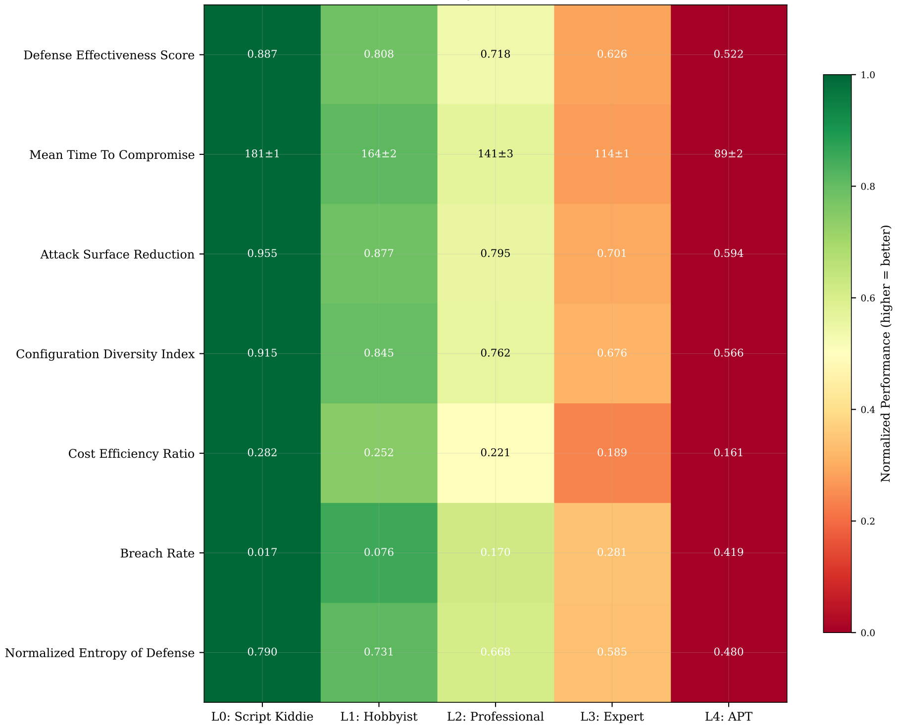
Final Performance by Attacker Level and Metric
