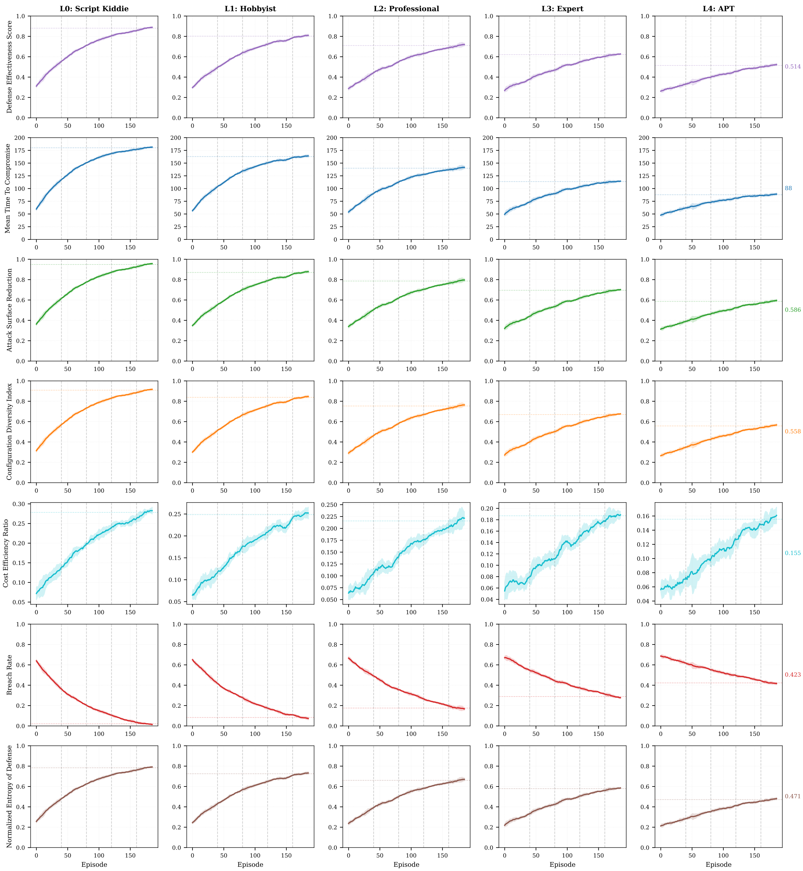
Training Convergence by Attacker Sophistication Level (95% CI shaded)
