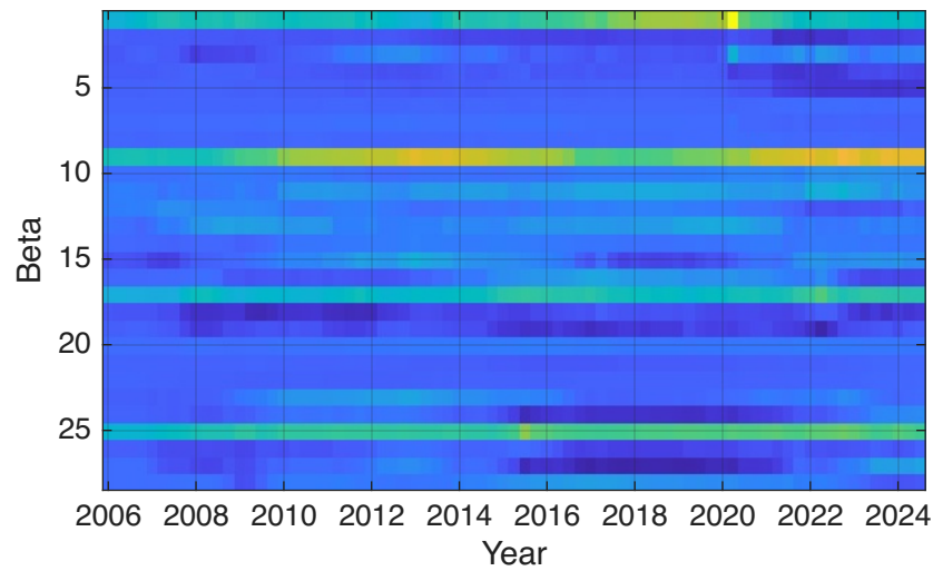
Kalman Filter
