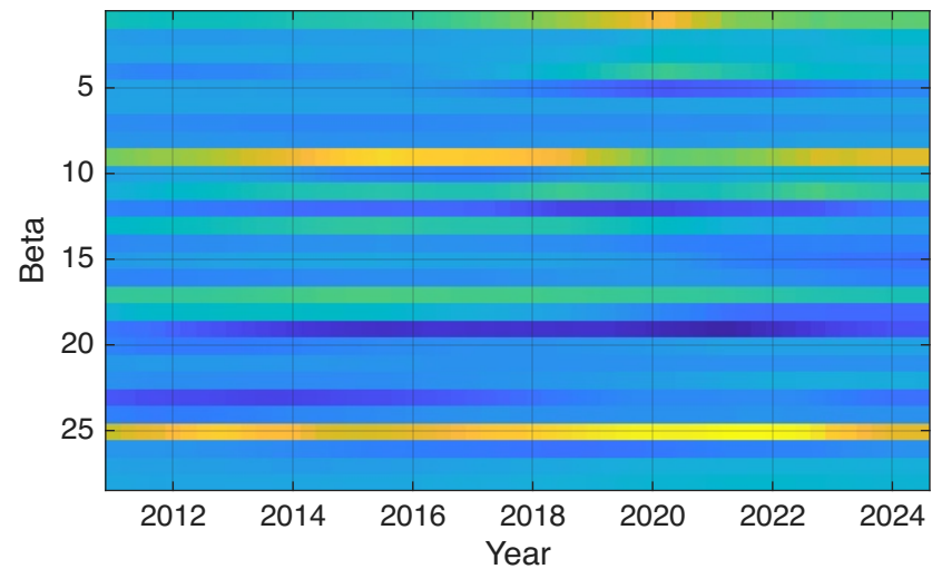
Kalman Smoother
