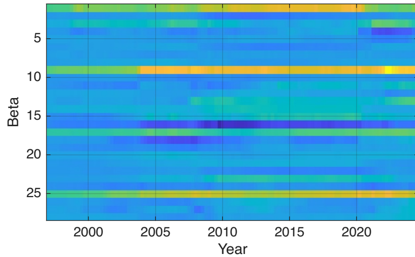
Kalman Filter
