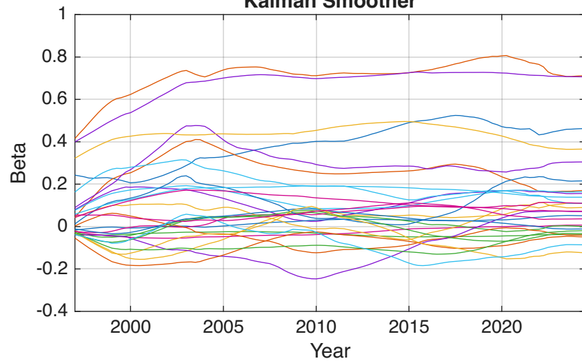
Kalman Smoother
