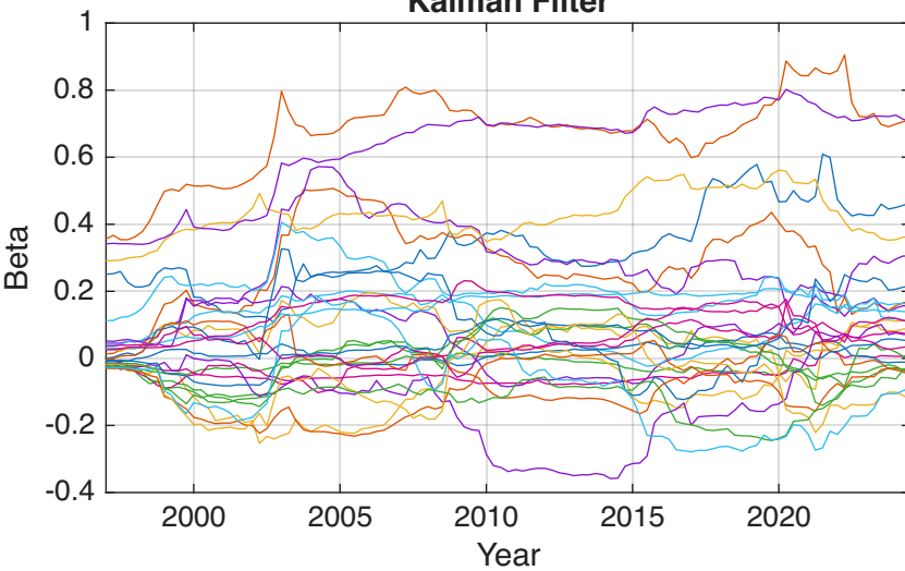
Kalman Filter
