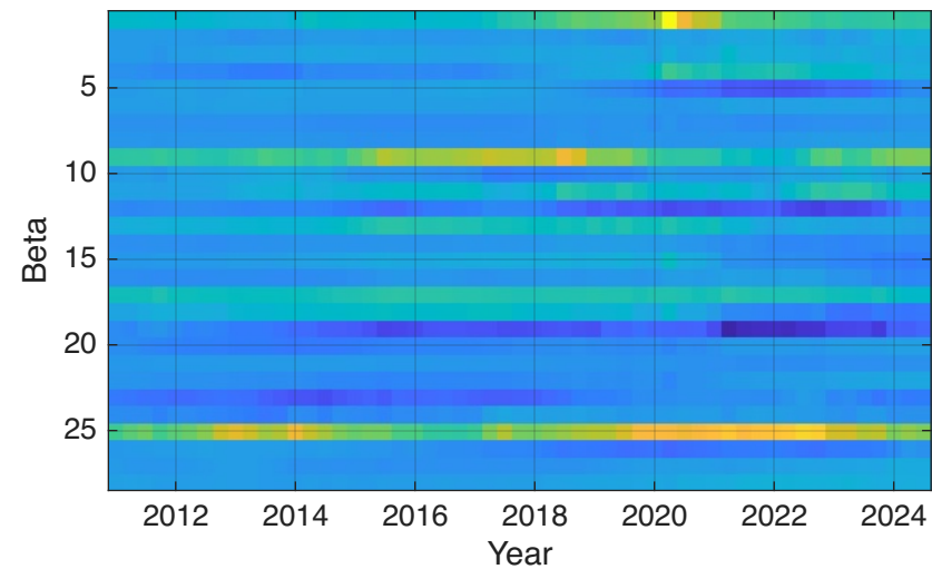
Kalman Filter
