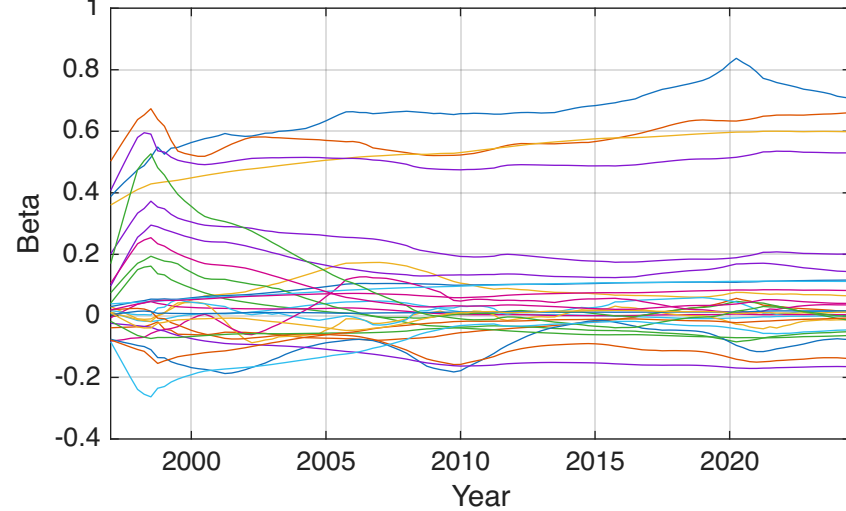
Kalman Smoother
