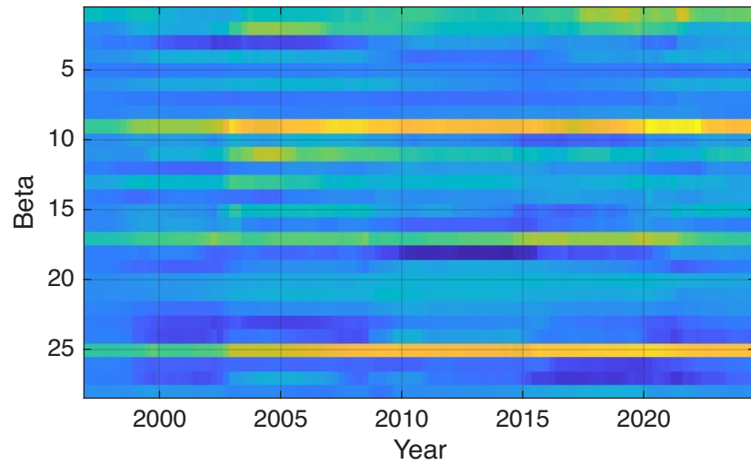
Kalman Filter
