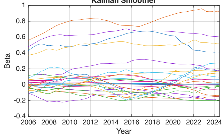
Kalman Smoother
