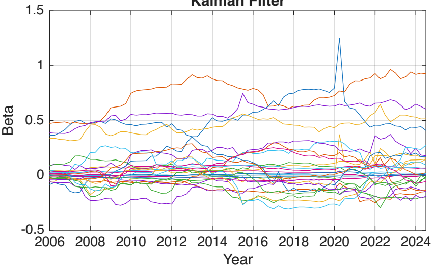
Kalman Filter
