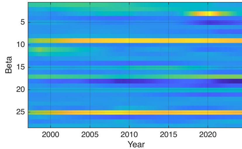
Kalman Smoother
