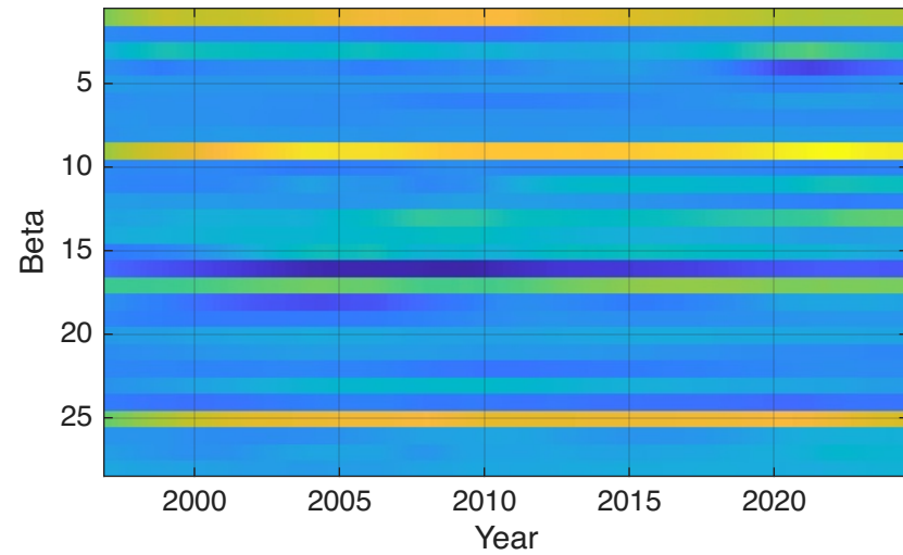
Kalman Smoother
