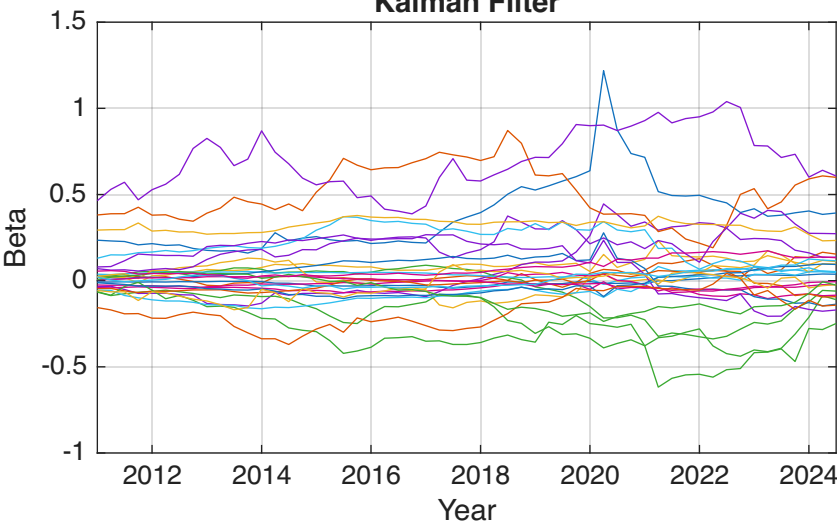
Kalman Filter
