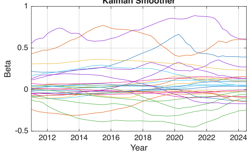
Kalman Smoother
