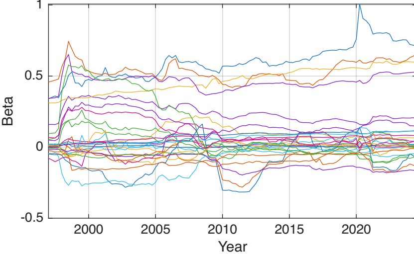
Kalman Filter
