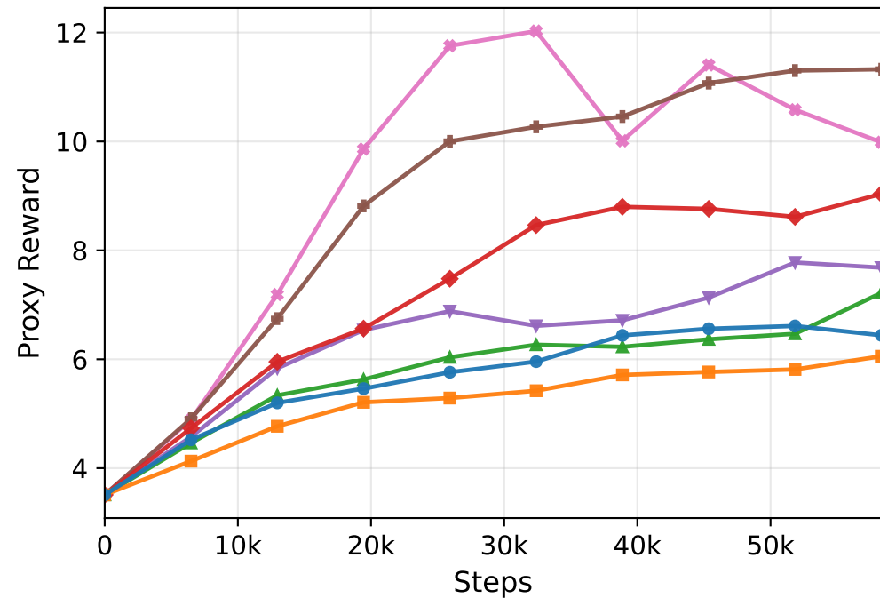
(a) Proxy Reward
