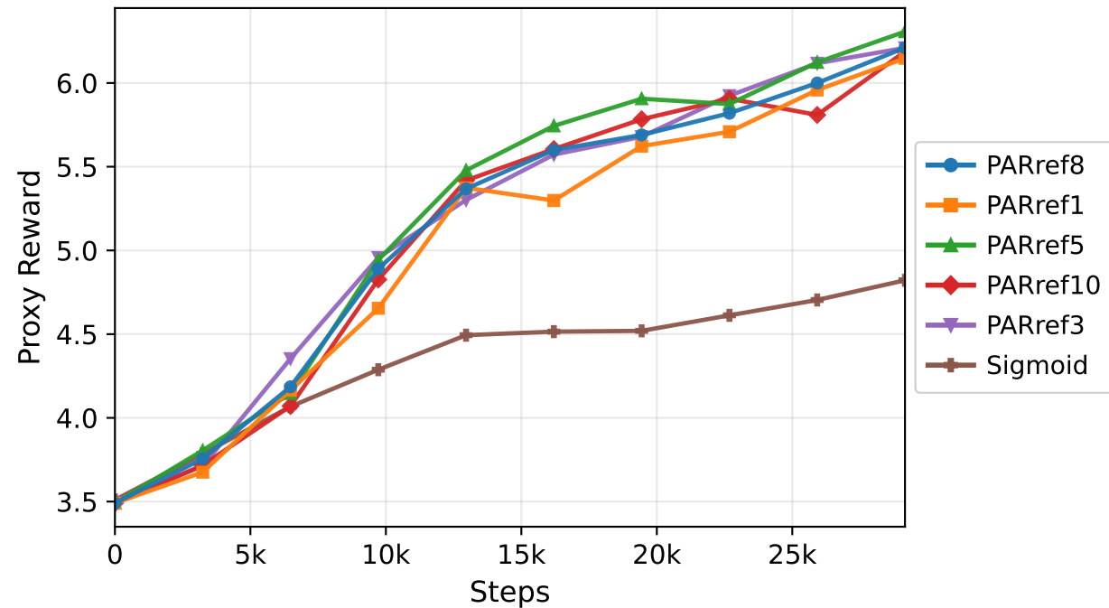
(a) Proxy Reward
