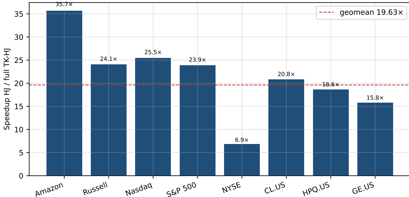
Per-dataset speedup at the central configuration
