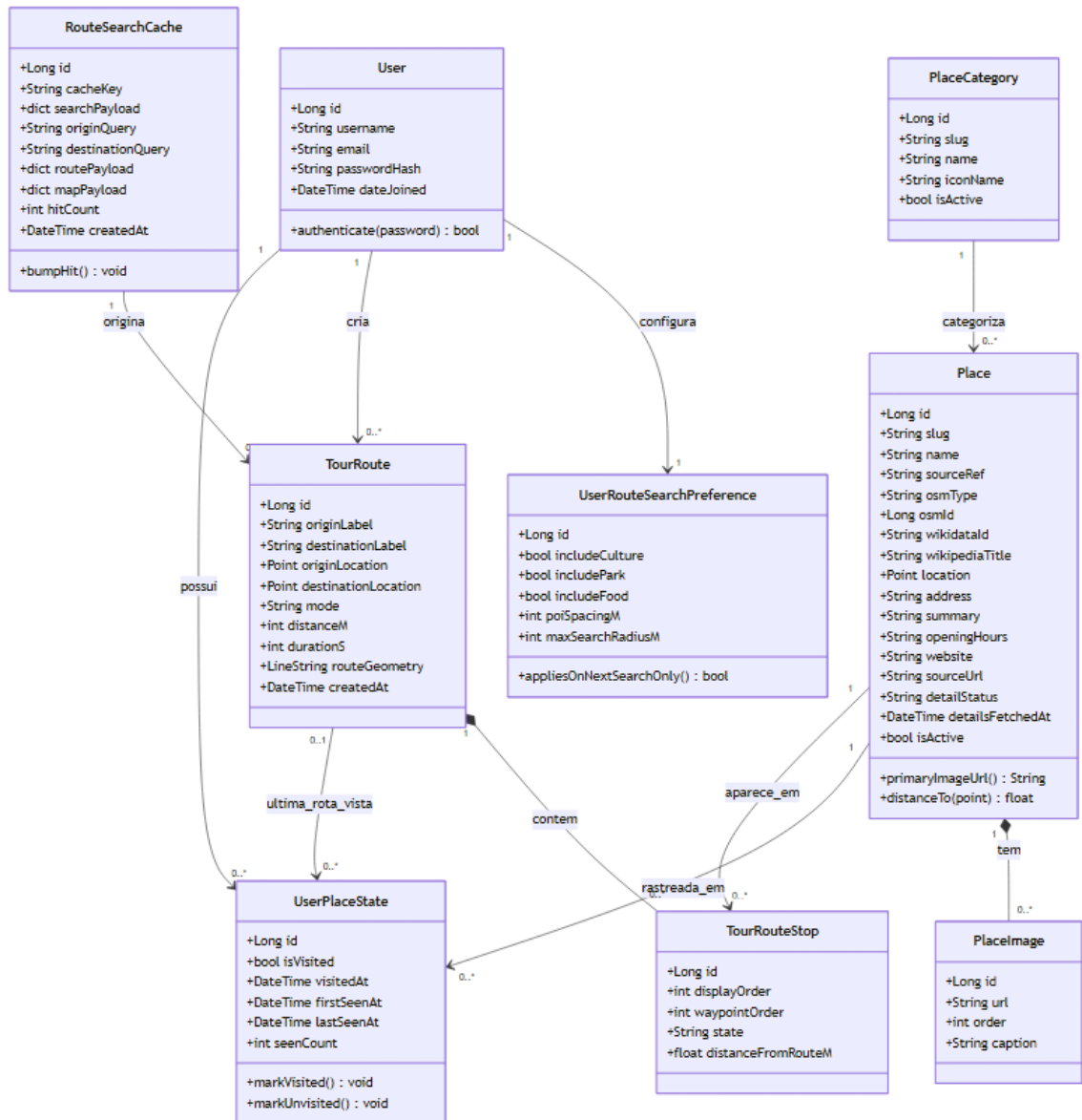
Figura 4: Diagrama de classes principal
