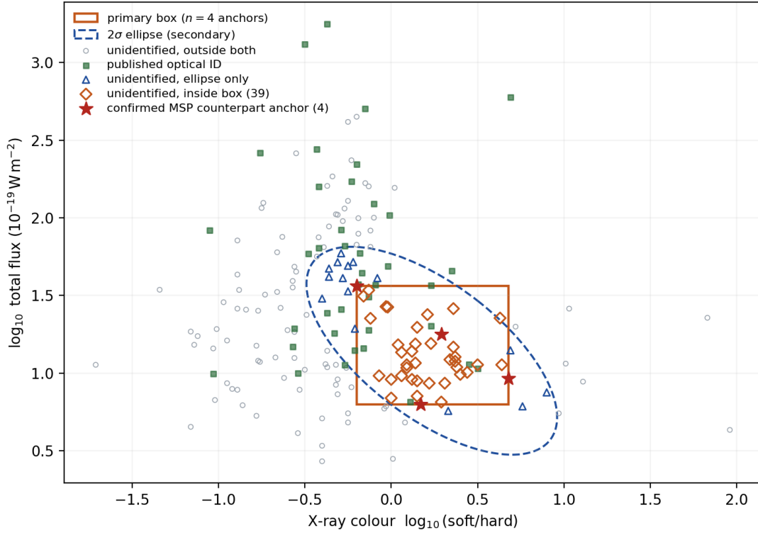
Figure 7: The colour-flux plane inside the 480'' aperture, with the primary bounding box and the secondary 2\sigma ellipse drawn on the four confirmed counterparts that anchor them. Both regions are constructed from the four stars plotted inside them, so the anchors' position in the region is a construction and not a test of it. The box holds 39 unidentified sources and the ellipse 53, and neither screens for background AGN, which is why both counts are upper bounds. Twelve aperture sources lack a colour or a flux and do not appear. Values from figs/fG_expand.colourflux.json .
