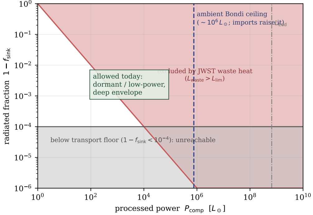
Figure 2: The (P_{\text{comp}}, 1 - f_{\text{sink}}) constraint plane for an \omega Cen installation. Red: excluded by the JWST mid-infrared point-source limit. Grey: below the entropy-transport floor. Dashed: the ambient Bondi fuel ceiling ( \sim 8 \times 10^5 L_{\odot} ; imported mass moves it right at the cost of visibility). The surviving region is dormant or low-power and deep.
