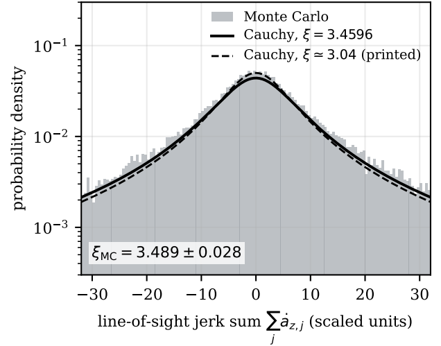
Figure 1. Route (iii). Line-of-sight jerk sums from 4 \times 10^4 realizations of a Poisson stellar field with Maxwellian velocities, in the scaled units G = \langle m \rangle = \sigma = n = 1 , against the Cauchy law of Prager et al.’s Equation B10 at the corrected scale ( \xi = 3.4596 , solid) and the printed scale ( \xi \approx 3.04 , dashed). The interquartile estimate for this sample is \xi_{\text{MC}} = 3.4886 \pm 0.0283 , excluding 3.04 at 15.8\sigma .
