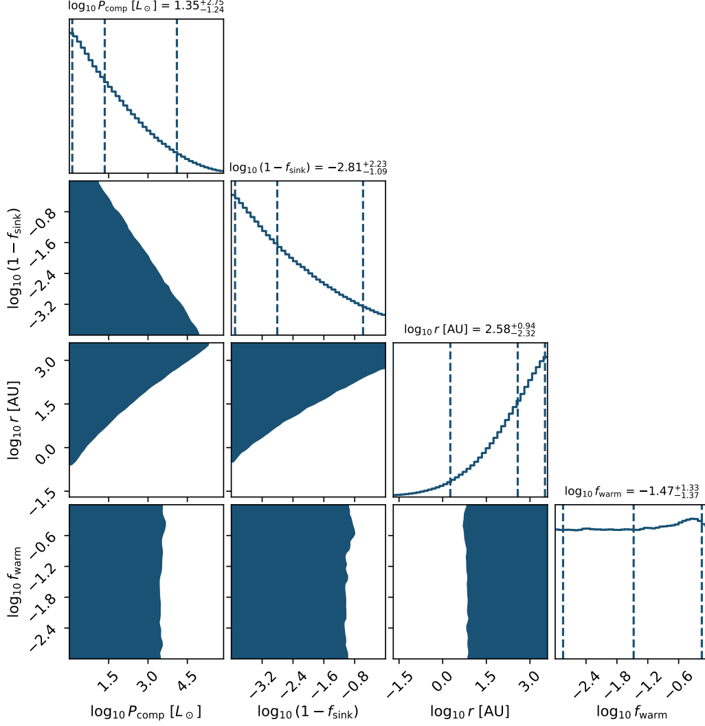
Figure 5: Posterior corner plot of the active-installation parameters under the priors above and the v1.0 continuous MIRI likelihood at the 2026 limits (crowding \times 3 ; the same 2 \times 10^6 -draw run as the table). The posterior is the prior times the binary detection likelihood — a configuration contributes iff its two-temperature SED evades every MIRI filter — so the corner displays the surviving prior volume: which parameter combinations the 2026 limits exclude and which survive. The surviving mass sits at low P_{\text{comp}}(1 - f_{\text{sink}}) (the deeply sub-Eddington corner), at large swarm radii (cool SEDs), and is nearly independent of the warm/cool split f_{\text{warm}} , which the on-off detection structure barely constrains. The excluded 75.5 per cent of the prior volume ( \xi = 0.755 ) is the complementary high-luminosity, small-radius region.
