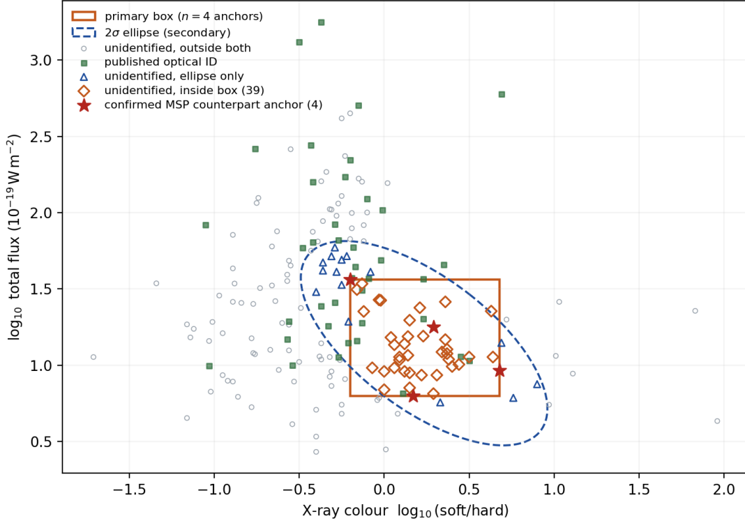
Figure 6: The colour-flux plane inside the 480'' aperture, with the primary bounding box and the secondary 2\sigma ellipse drawn on the four confirmed counterparts that anchor them. Both regions are constructed from the four stars plotted inside them, so the anchors' position in the region is a construction and not a test of it. The box holds 39 unidentified sources and the ellipse 53, and neither screens for background AGN, which is why both counts are upper bounds. Twelve aperture sources lack a colour or a flux and do not appear. Values from figs/fG_expand_colourflux.json .
