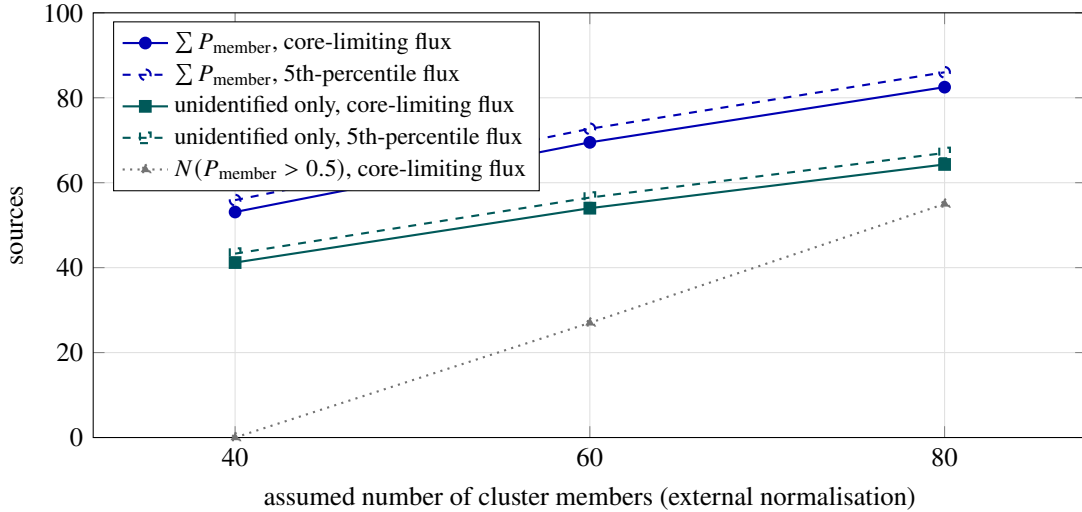
Figure 4: Membership ladder. Summed membership probability over the 480'' aperture, and over its unidentified subset, against the assumed external member normalisation at two background flux limits. The count of sources individually exceeding P_{\text{member}} = 0.5 (dotted) moves from 0 to 55 over the same range, which is why membership is reported as a summed probability under stated assumptions and not as a label. Values from analysis/results_omega_cen.json.
