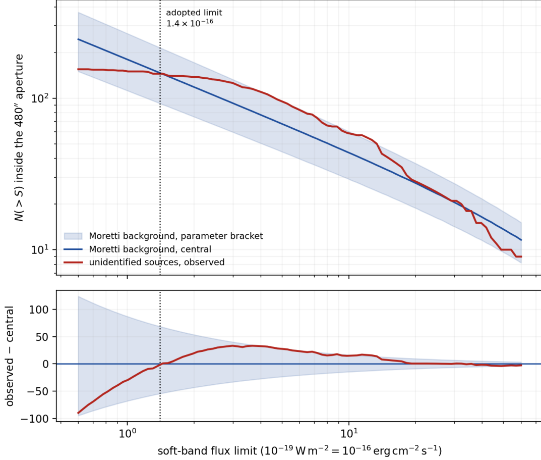
Figure 5: The residual, drawn rather than quoted. Top: cumulative count of unidentified sources inside the 480'' aperture above a soft-band flux limit, against the Moretti et al. (2003) background expectation over the same solid angle with its published parameter uncertainties propagated as a bracket. Bottom: the same difference on a linear scale. The observed curve stays inside the bracket at 90 per cent of the sampled limits; where it crosses the upper edge, between 4 and 13 \times 10^{-16} \text{ erg cm}^{-2} \text{ s}^{-1} , it does so by at most 2.1 sources against a Poisson error of 7.5 on the count there, so the crossing carries no excess. The faint-end flattening of the observed curve is catalogue incompleteness. Values from figs/fg_expand_lognlogs.json .
