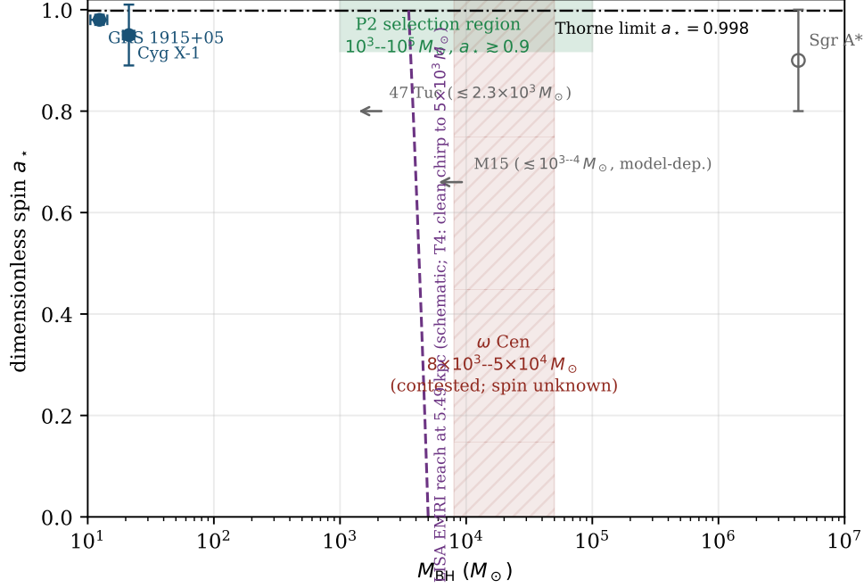
Figure 2: The mass–spin plane. Blue: stellar-mass black holes with spin measurements (representative continuum-fitting values; compilation in Reynolds 2021). Red hatched band: the contested \omega Cen central mass, 8 \times 10^3 – 5 \times 10^4 M_\odot (Table 6), spin unknown. Grey arrows: IMBH candidates constrained only from above (47 Tuc, Kızıltan et al. 2017; M15, Greene et al. 2020). Grey open symbol: Sgr A* (spin inferred; GRAVITY Collaboration 2022). Green: the P2 selection region, 10^3 – 10^5 M_\odot at a_\star \gtrsim 0.9 (criteria 1–2). Dash-dotted line: the Thorne (1974) spin-equilibrium limit a_\star = 0.998 . Dashed curve: schematic LISA EMRI mass reach at 5.49 kpc, anchored at the T4 threshold of 8.2 \times 10^3 M_\odot (Table 7) and drawn slightly deeper at high spin, where the inspiral spends more cycles in band. The curve states a requirement the test places on LISA, not a demonstrated reach at this distance; no mission-level sensitivity study for cluster EMRIs at 5.49 kpc is cited here, and the threshold should be read as the mass resolution T4 would need.
