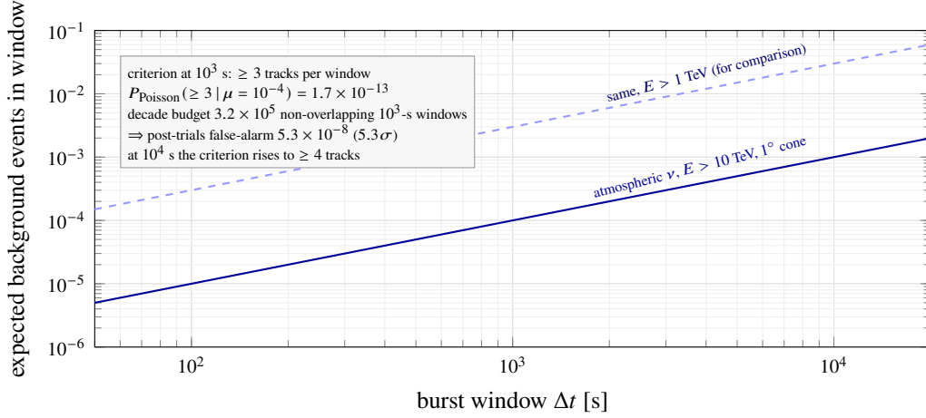
Figure 3: Design of the neutrino burst search. Expected atmospheric-neutrino background within 1° of \omega Cen versus window length, for the working E > 10 TeV threshold (solid) and a softer 1 TeV threshold (dashed). At 10 3 s the expectation is \sim 10^{-4} events, so the triplet criterion clears 5\sigma post-trials at 10 2 and 10 3 s under the 20× envelope; at 10 4 s it reaches only 4.4\sigma against that envelope, which is why the pre-registered multiplicity rises to four tracks in the longest window. Rate normalizations are order-of-magnitude, with exact values set by the detector Monte Carlo at analysis time.
