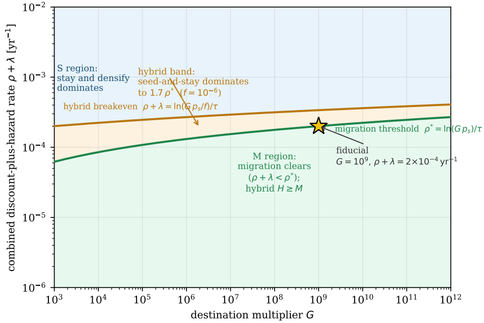
Figure 3: The phase space of the migration decision in the (G, \rho + \lambda) plane, at p_s = 0.5 and \tau = 10^5 yr (Table 1). Green: migration clears, \rho + \lambda < \rho^* = \ln(G p_s)/\tau (Eq. 9); within it the hybrid weakly dominates pure M under the seed-fidelity assumption. Orange: the hybrid band, where the hybrid beats S while pure M does not, extending to \rho + \lambda = \ln(G p_s / f)/\tau = 1.7 \rho^* at the fiducial seed cost f = 10^{-6} (Eq. 11). Blue: S dominates; neither migration nor seeding pays. The star marks the fiducial point ( G = 10^9 , \rho + \lambda = 2 \times 10^{-4} \text{ yr}^{-1} ), which sits on the migration threshold.
