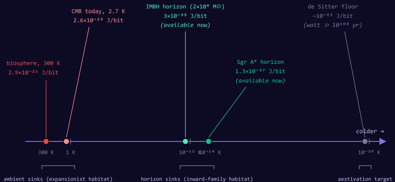
Figure 1. The entropy-sink hierarchy: minimum erasure cost k_{\text{B}}T \ln 2 versus sink temperature (logarithmic axis, temperature decreasing rightward). The inward family's central observation is that horizon sinks colder than any achievable future CMB exist in the present epoch ; the aestivation strategy of waiting for the de Sitter floor (Sandberg et al. 2016) buys \sim 18 further decades of efficiency at the price of \gg 10^{100} years and the free-energy losses identified by Bennett et al. (2019).
