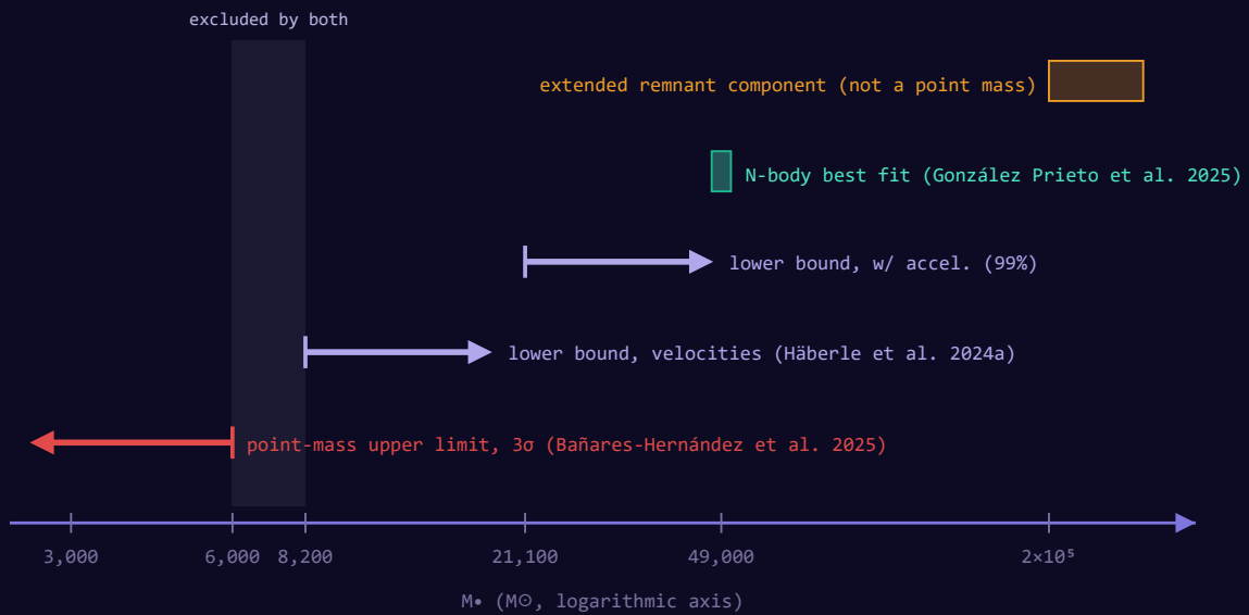
Figure 1. The central-mass constraint landscape (logarithmic mass axis). The pulsar-timing point-mass upper limit and the fast-star kinematic lower bounds leave no allowed point mass: at least one constraint must yield. The campaign is structured to determine which, on a known schedule, using instruments that share no dominant systematics.
