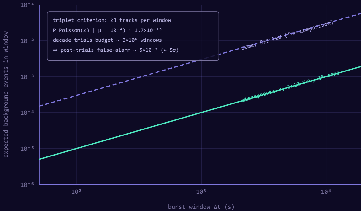
Figure 3. Design of the neutrino burst search. Expected atmospheric-neutrino background within 1^\circ of \omega Cen versus window length, for the working E > 10 \text{ TeV} threshold (solid) and a softer 1 \text{ TeV} threshold (dashed). At 10^3 \text{ s} the expectation is \sim 10^{-4} events, so the pre-registered triplet criterion is intrinsically
