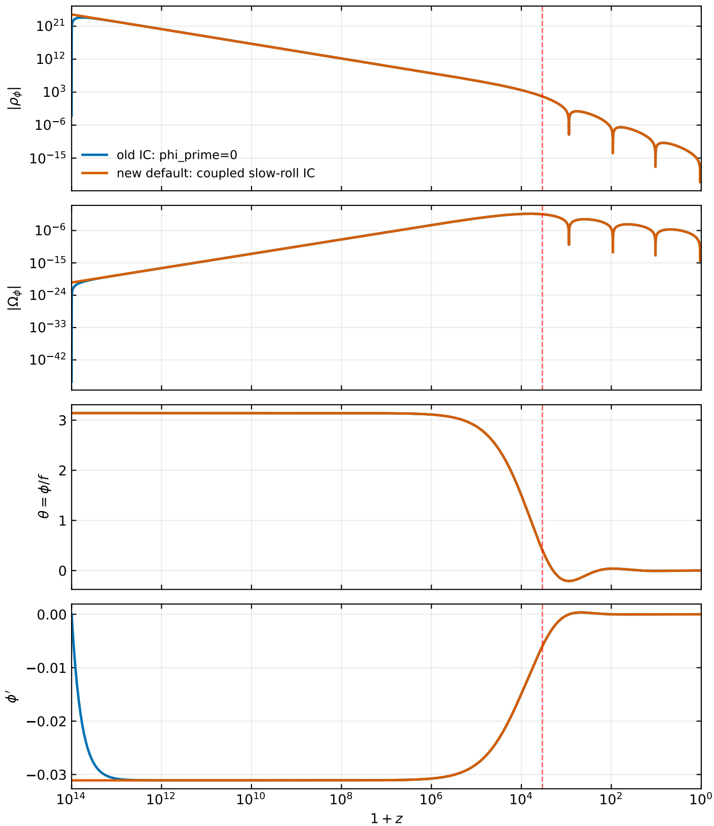
Coupled IC comparison: f = 0.5 , m/H_0 = 100 , g = 1
