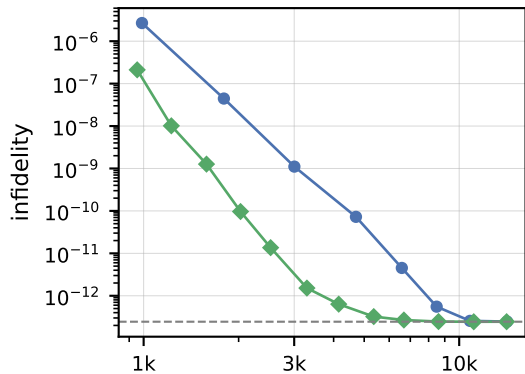
spin-boson d = (32, 16, 16, 16)
