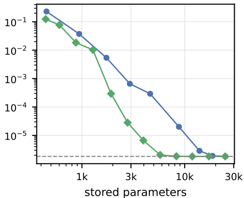
pyrazine
