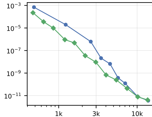
spin-boson d = (8, 8, 8, 8, 8, 8)
