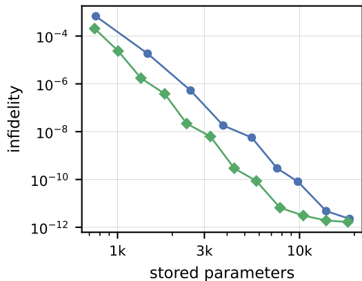
spin-boson d = (64, 32, 16, 8, 4, 2)
