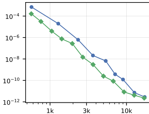
spin-boson d = (24, 16, 12, 8, 6, 4)
