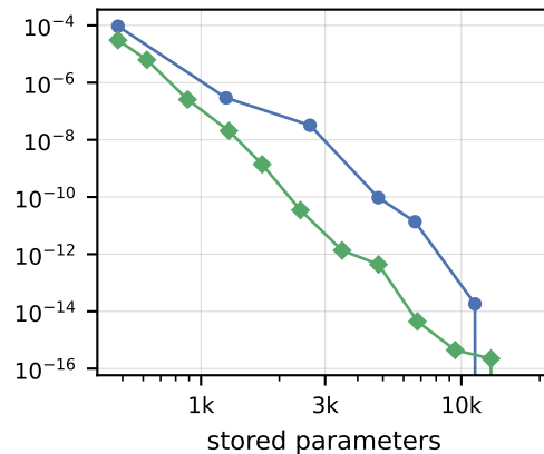
Holstein chain
