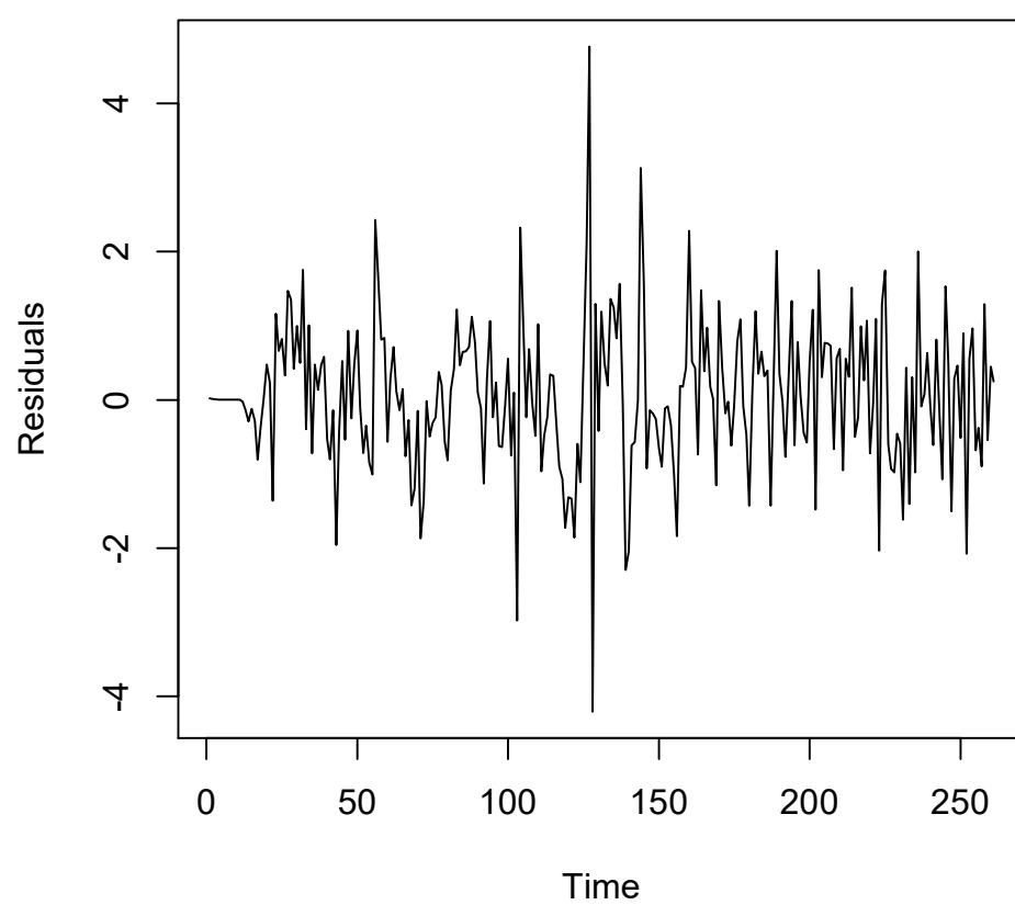
Plot of residual series of ARIMA(2,1,2,2,1,1,12)
